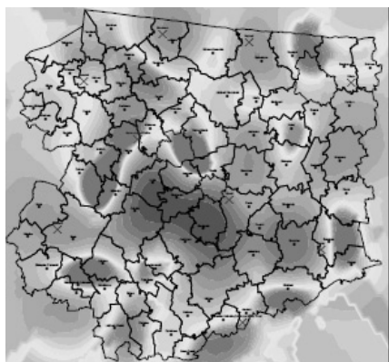
a) metoda Kriging Ordinary
